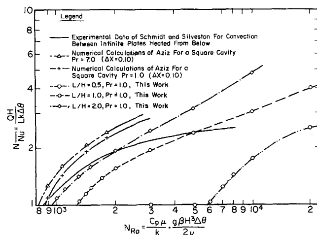
Fig. 5. Comparison of the results of this investigation with the calculations of Aziz and the data of Schmidt and Silveston.
